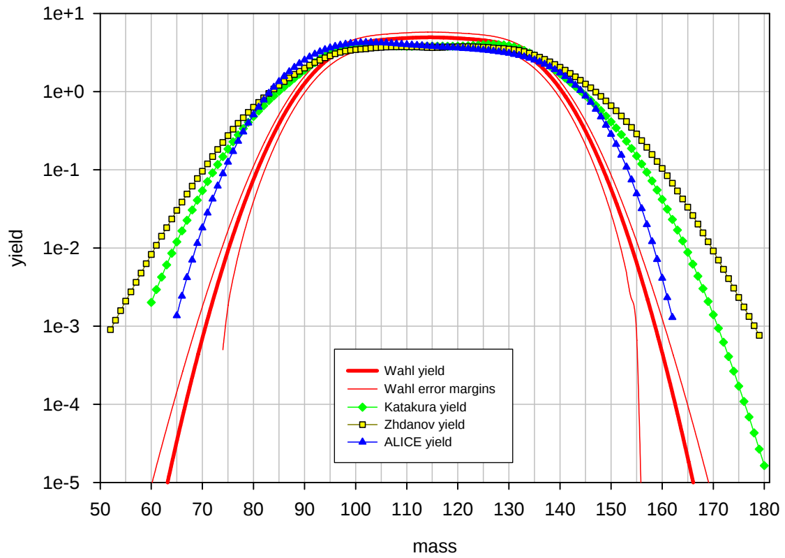
Benchmark B: ^{241}\text{Am} at 160 MeV, post neutron emission mass distribution
